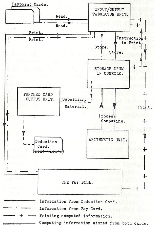
A Block Diagram of the Computer used by the "Western Region".
